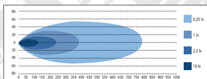
W-LIGHT IMPULSE II 528 mm
