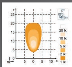
Nordic Lights KL2001 20 W
