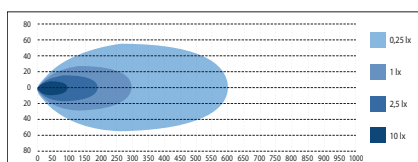
W-LIGHT STORM 10 306 mm. Parktuli
