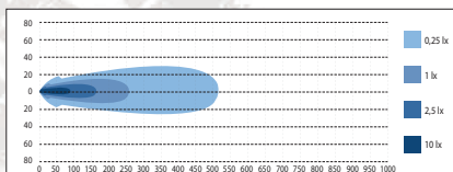
W-LIGHT HURRICANE 200 200 mm
