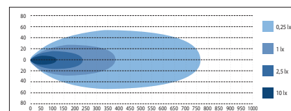
W-LIGHT BLIZZARD SLIM 494 mm
