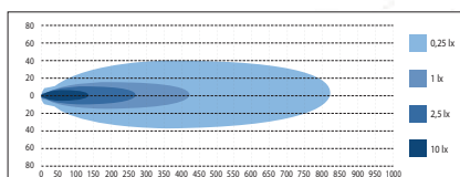
SEEKER X 429 mm. Parktuli
