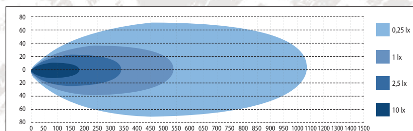
W-LIGHT IMPULSE III 527 mm
