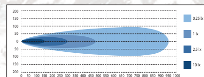
X-VISION GENESIS 600 561 mm
