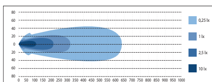
W-LIGHT HURRICANE 400 357 mm
