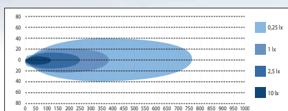
X-VISION GENESIS 300 314 mm
