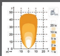
Nordic Lights Pictor 620 28 W
