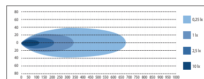
W-LIGHT RIPPLE 360 SLIM 360 mm
