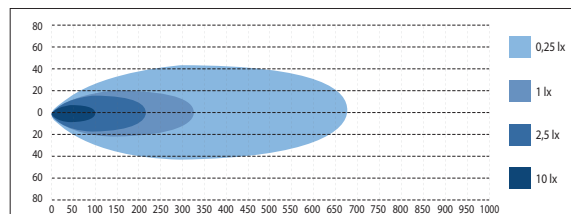
W-LIGHT IMPULSE I 360 mm
