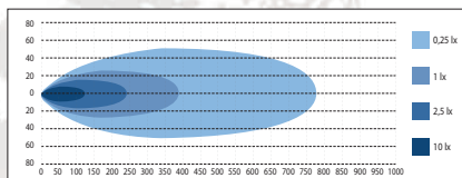
W-LIGHT RIPPLE 530 528 mm
