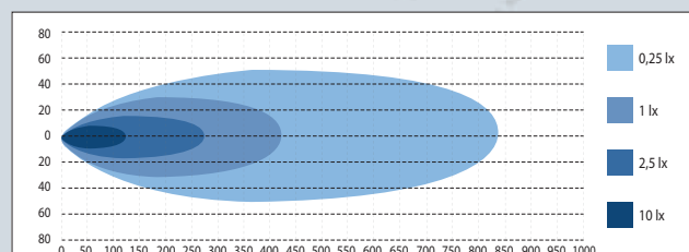
X-VISION OPTIMA 12 584 mm
