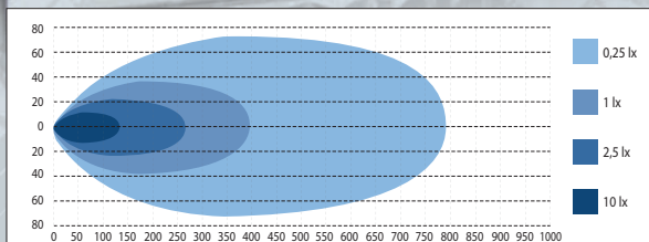
W-LIGHT STORM 20 486 mm. Parktuli
