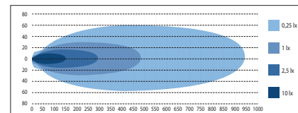
W-LIGHT WAVE 532 mm
