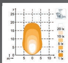
Nordic Lights Scorpius GO 420 28 W
