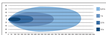
X-VISION D-MaXX 527 mm
