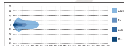
W-LIGHT SIDE SHOOTER 253 mm. Soojendatav klaas, side
