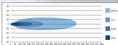
SEEKER X 245 mm. Parktuli
