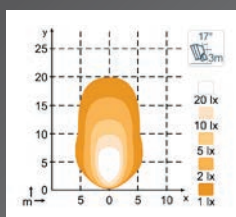
Nordic Lights Canis GO 420 28 W
