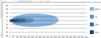
W-LIGHT NEPTUNE III Parktuli
