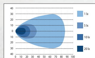
BULLPRO CENTUM 4500 K 100 W
